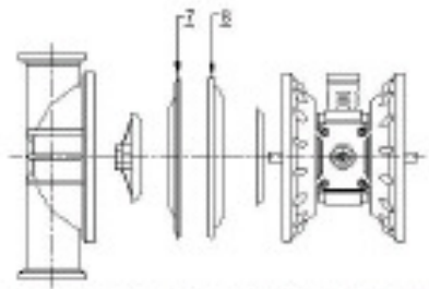
BACKUP DIAPHRAGM IS PROVIDED WITH TEFLON DIAPHRAGM
